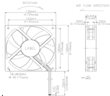
DIMENSION DRAWING
